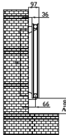
VLND Side View
