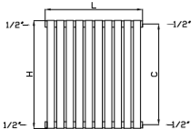
LND Front View
