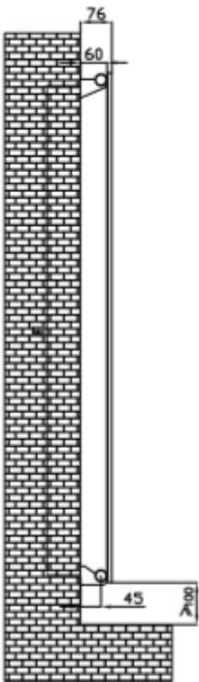
VLNS Side View
