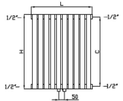
VLND Front View
