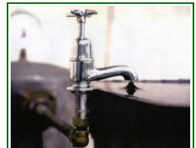
This tap is sucking up potentially contaminated fluid because there is insufficient air gap
