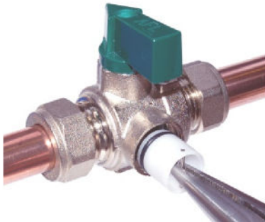
There are 8 colour-coded AFL cartridges that fit into valve in-situ . Cartridge fits into centre of ball via side port – no need to isolate or drain supply . Pliers can be used to remove cartridge. A cartridge can be fitted or changed in less than a minute
