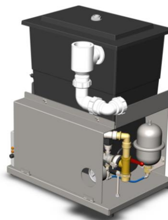
Home Water Booster Pump – code BTSBBPV3-3
