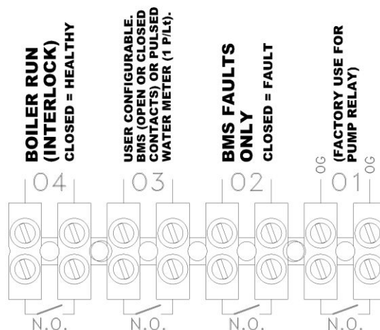
CONTROL TERMINALS AM176*
