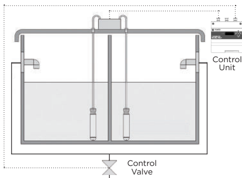
Balanced Tanks
