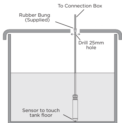
Single Tank
