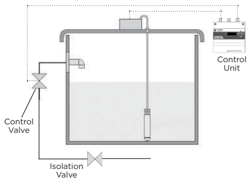
Single Tank
