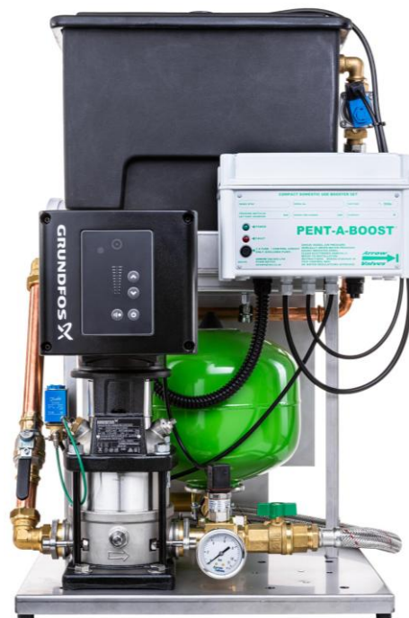
Model 5-8 - Quiet variable speed. Height 765 mm. High flow pump – single pump range up to 2 Lt/s output
