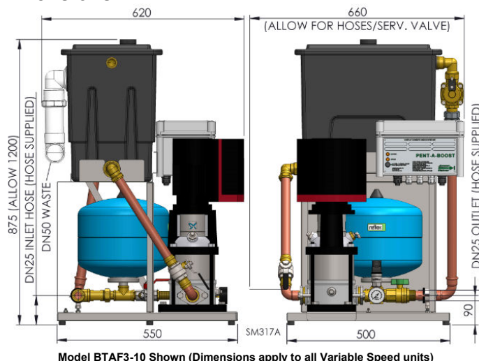
Model BTAF3-10 Shown (Dimensions apply to all Variable Speed units)
