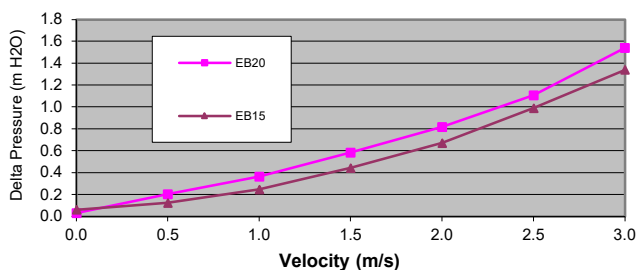
Head Loss / Flow Chart Model EB235
